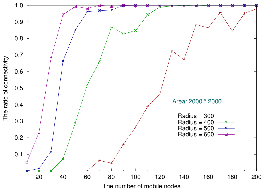
Figure 3: MANET connectivity
